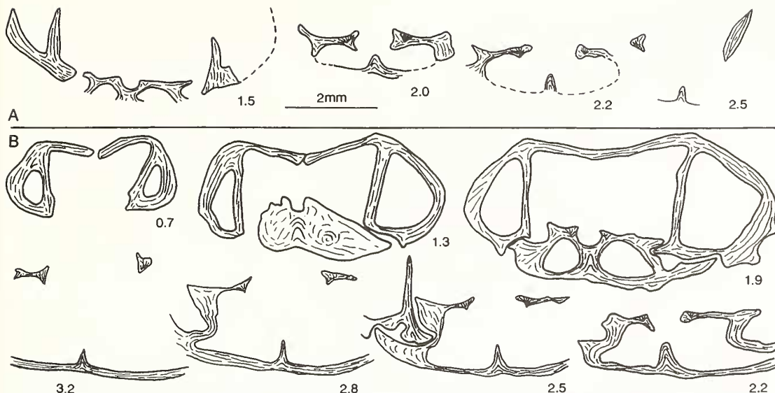
TEXT-FIG. 11. Transverse serial sections of biplicate Y. hanburyi Morphotype 1. Numbers refer to distance in mm from ventral apex. A, sample C-H, PUM92059. B, sample L12/0-0-1, PUM92060 (shell compressed).
